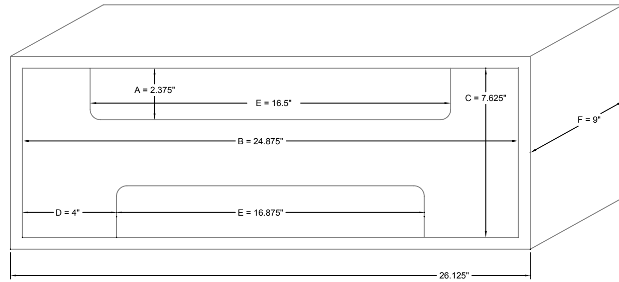
Small box cab will fit Weber 6M45 chassis styles or types
