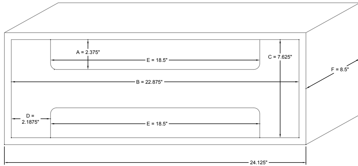
18 watt cab and will fit GDS chassis styles or types
