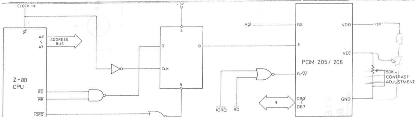
Figure 2. Module Block Diagram
