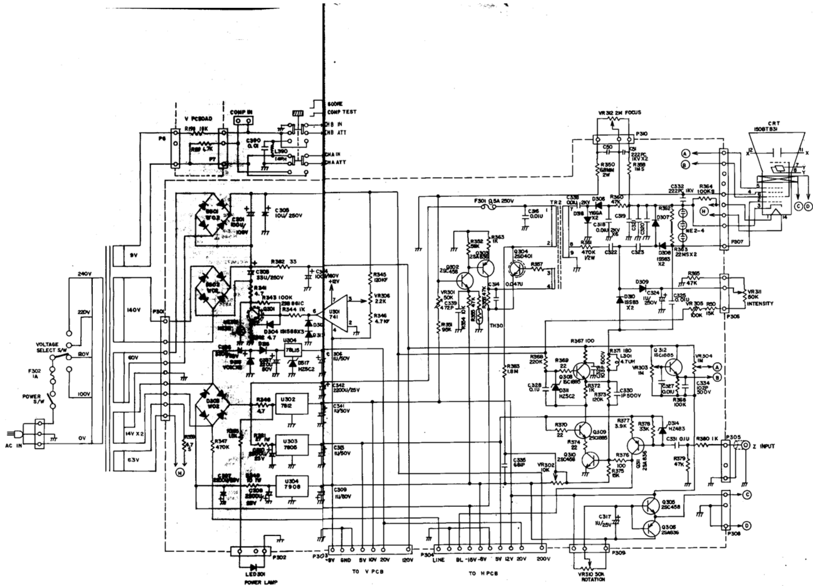
7-3 POWER SUPPLY CIRCUIT DIAGRAM
